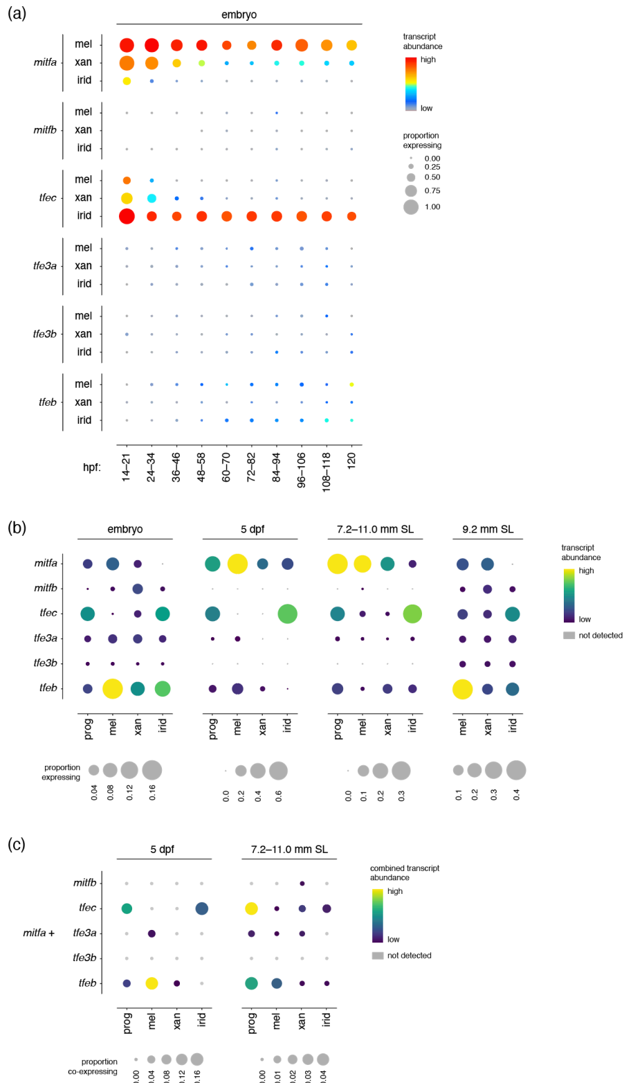
FIGURE S7 | Expression of mitfa and other MiT subfamily bHLH-ZIP transcription factor genes in published single cell transcriptomic datasets. Dot plots indicate transcript abundance and proportions of cells expressing mitfa and each of five MiT subfamily transcription factor genes. (a) Data for embryos at different hours post-fertilization (hpf) from daniocell.nichd.nih.gov (Sur et al., 2023). (b) Data from embryos (Saunders et al., 2023), 5 day post-fertilization (dpf) larvae and 7.2–11.0 mm standard length (SL) larvae (Saunders et al., 2019), and 9.2 mm SL larval skin (Aman et al., 2023). Note that published data sets for embryos in a and b are consistent with one another for some loci (e.g., mitfa and tfec ) and at variance with one another for other loci (e.g., mitfb , tfeb ). (c) Combined transcript abundances for cells identified to co-express mitfa with at least one other related transcription factor gene in single cell RNA-sequencing of Saunders et al. (2019) and Aman et al. (2023). Combined abundance of mitfa and tfec were particularly high for pigment cell progenitors.
