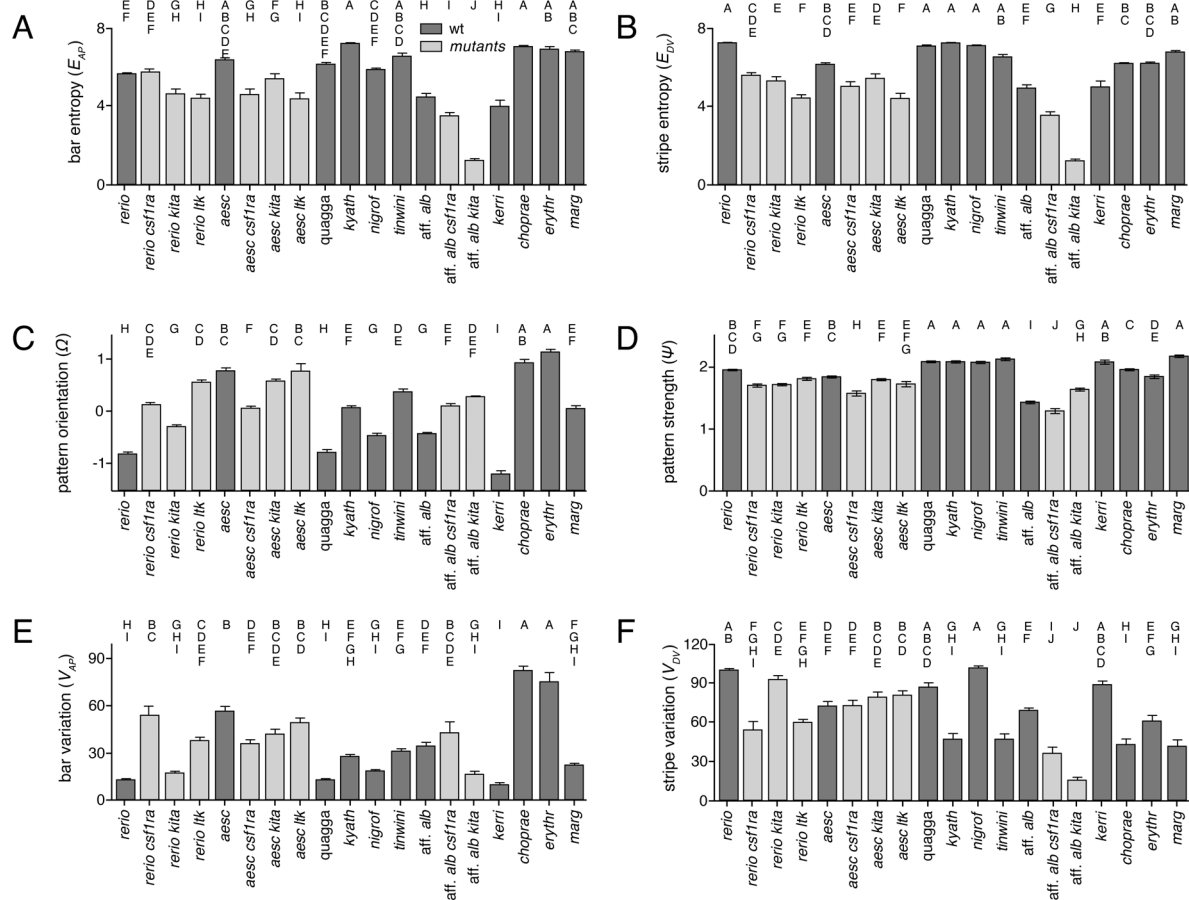
Fig. S3. Pattern metrics used in analyses. Shown are univariate plots (means±SE) for pattern metrics described in the main text. Dark grey bars indicate wild-types, light grey bars indicate csf1ra , kita , and itk mutants. Shared letters above bars indicate means that were not significantly different ( P > 0.05 ) in Tukey-Kramer post hoc comparisons (all ANOVA, P < 0.0001 ).
